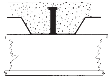
Typical metal deck with composite construction.
