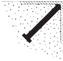
Typical loading dock embed plate.
